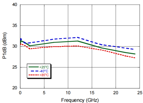
at 24V
